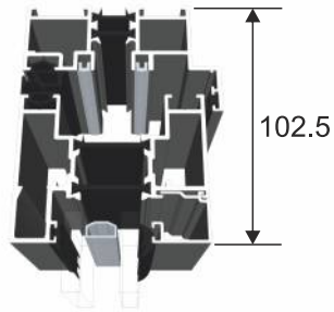
(B) Head
