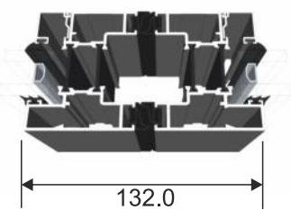
(C) Meeting Stile
