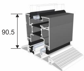
(E) 20mm Threshold
