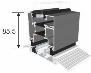
(F) 15mm Threshold
