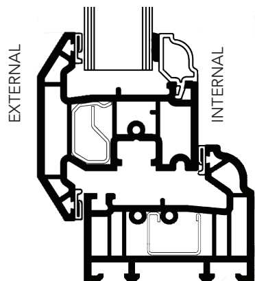
Heritage with Rebated Sash
